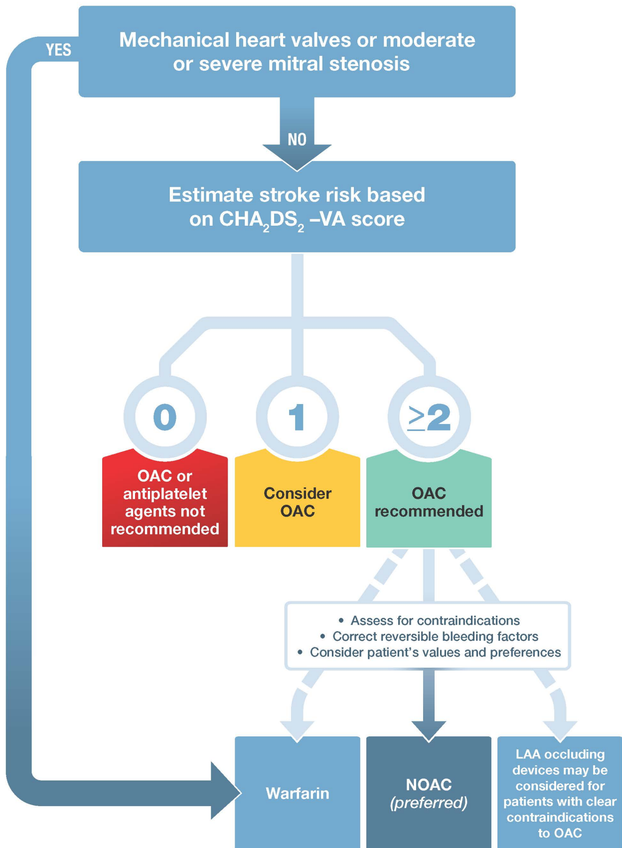
Figure 6: Stroke prevention in atrial fibrillation
